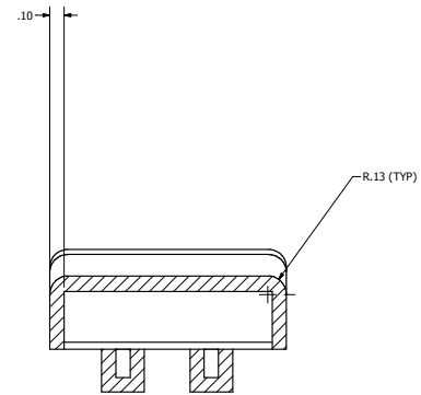
SECTION C-C SCALE 2.1
