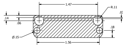
SECTION A-A SCALE 2.1
