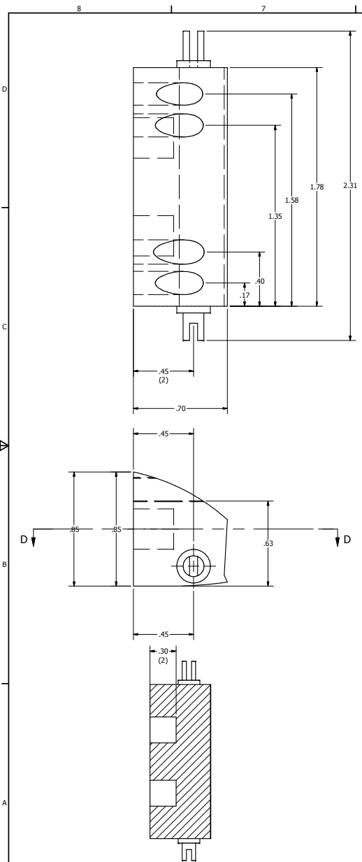
SECTION D-D SCALE 2/1
